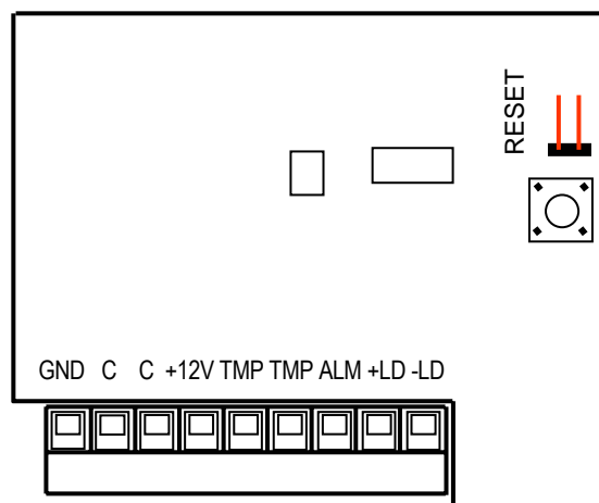
Fig. 2. Partial view of the PCB, version 2.1 (seen from the designations side).
